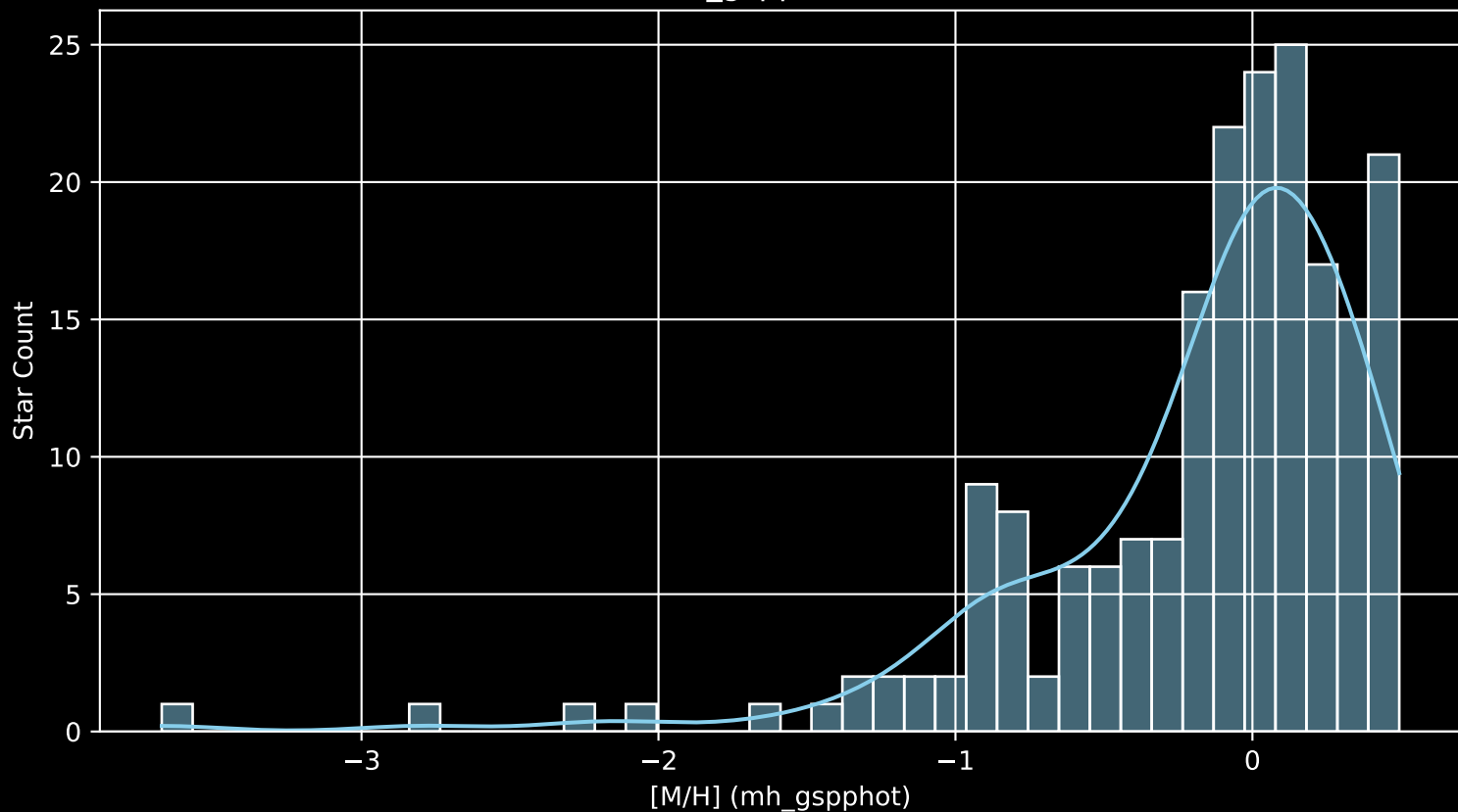
APOGEE DR17 Field: [049+00 [M/H] (mh_gspphot) (n= 199)
