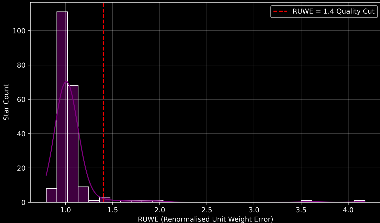
GAPOGEE DR17 Field [049+00] RUWE Distribution (n= 206)
