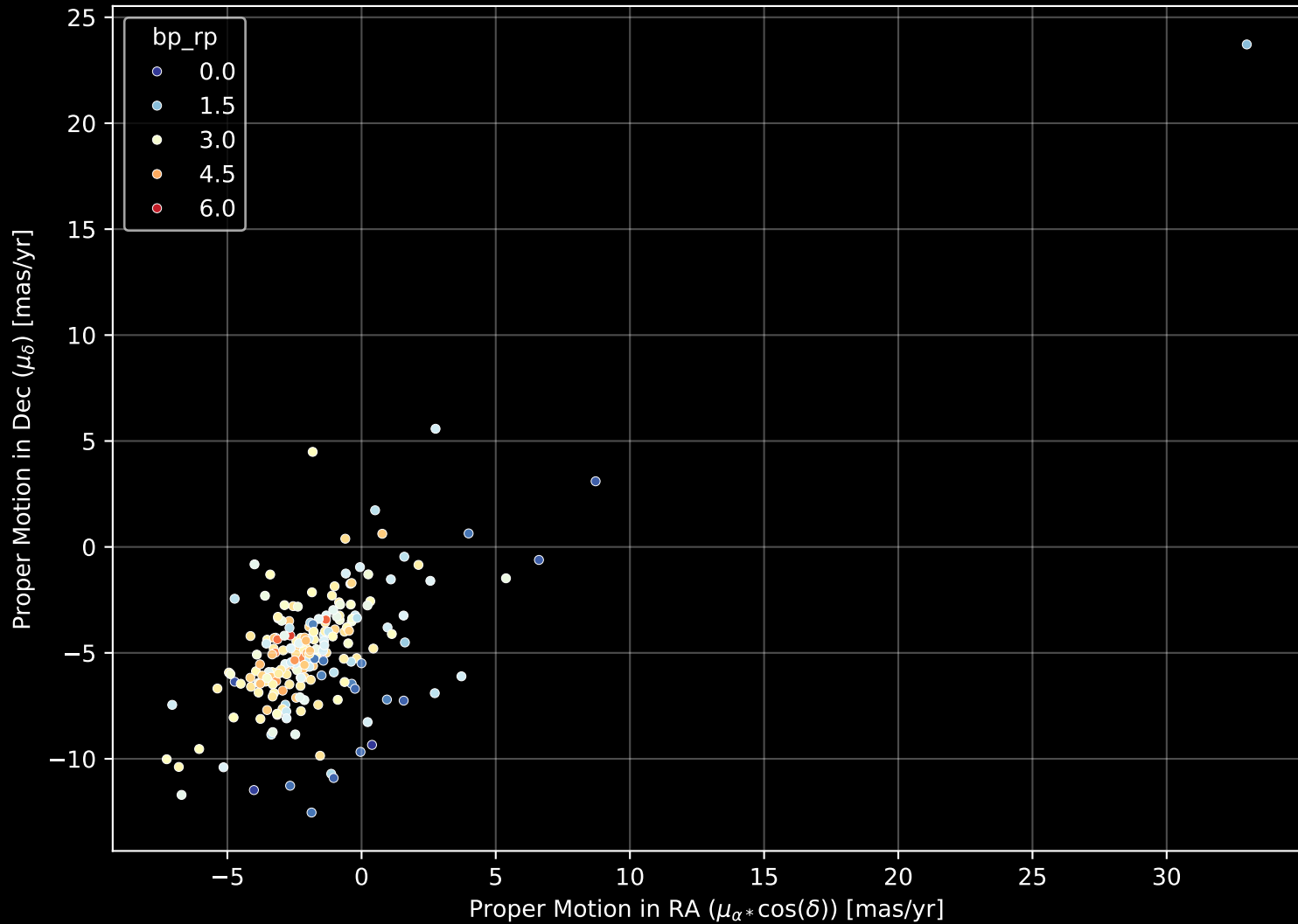
APOGEE DR17 Field: [049+00] Proper Motion Diagram (n= 209)
