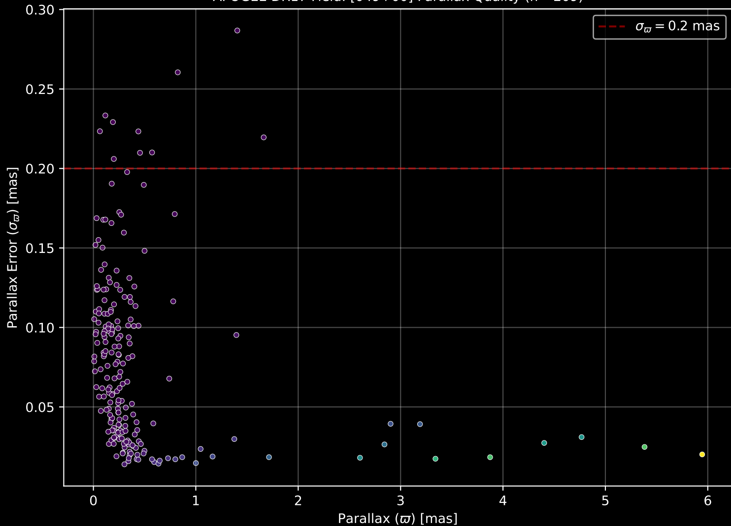
APOGEE DR17 Field: [049+00] Parallax Quality (n= 209)
