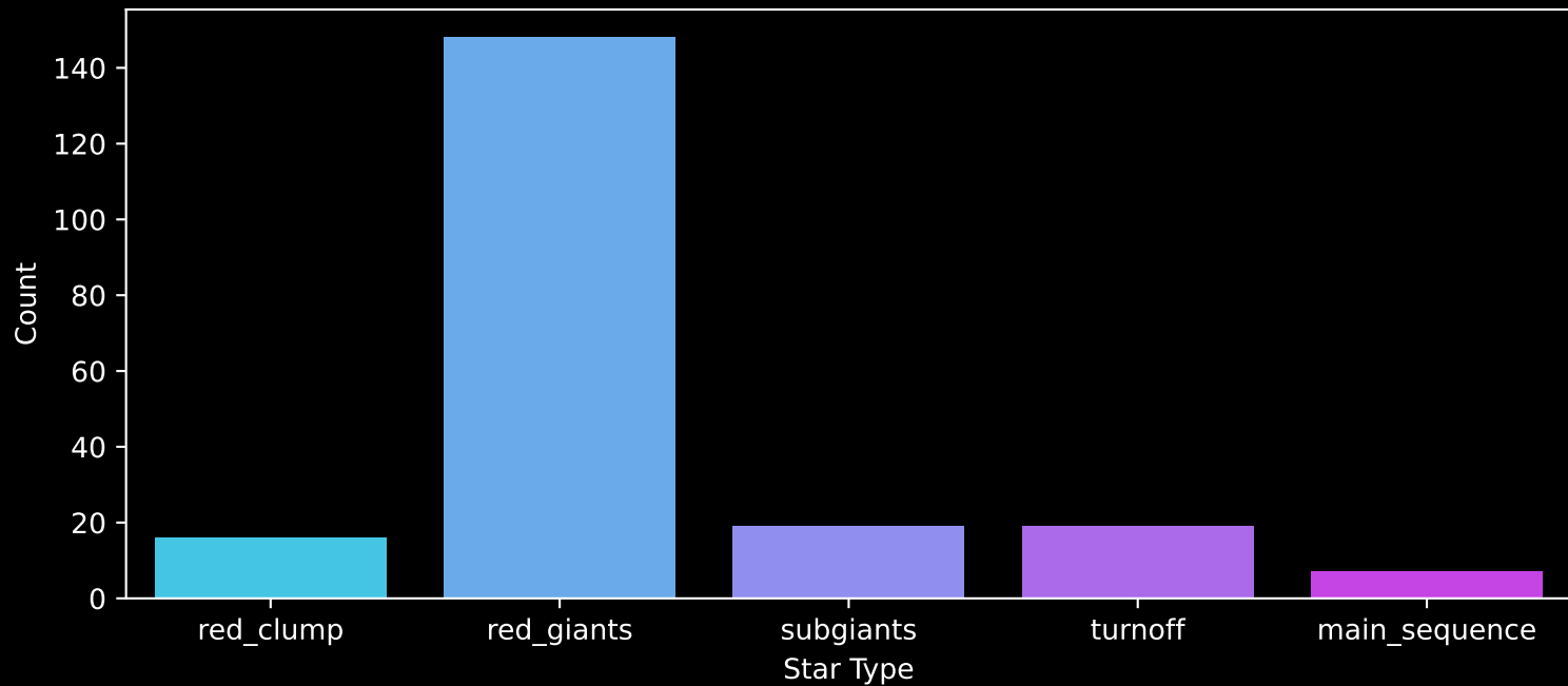
APOGEE DR17 Field: [049+00] Count plot of Star Type
